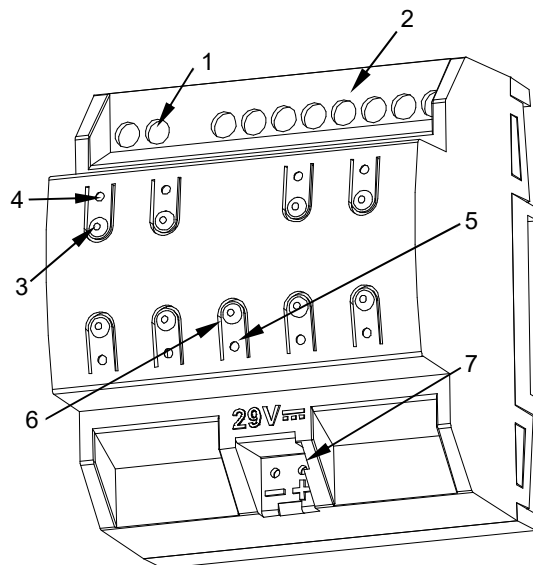
Figura 1: HeatingBOX 24V 8X
